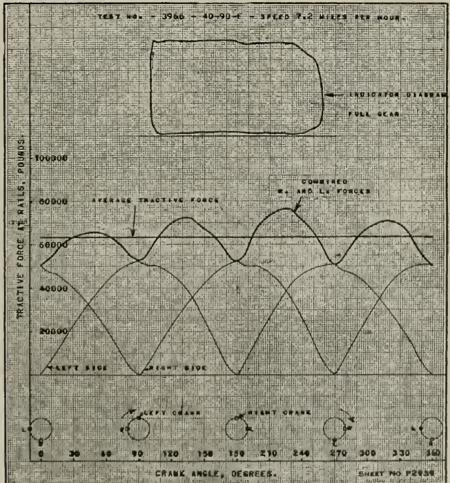
BELOW IS DIAGRAM OF TRACTIVE FORCE CURVES, FULL GEAR, CLASS 11S LOCOMOTIVES, CYLINDERS 27 X 30 INS., STEAM PRESSURE 205 LBS.
